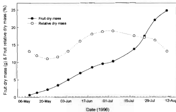
FIG. 2 Seasonal patterns of fruit dry mass and relative fruit dry mass for control treatment conditions and commercial crop load.
